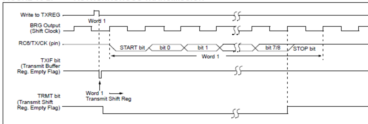
FIGURE 16-2: ASYNCHRONOUS TRANSMISSION
