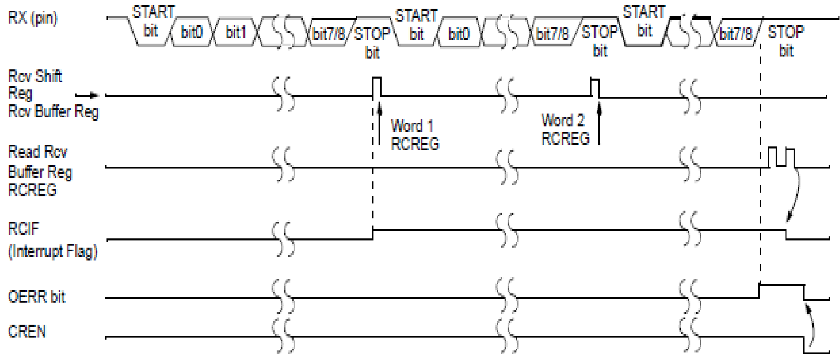
FIGURE 16-5: ASYNCHRONOUS RECEPTION
