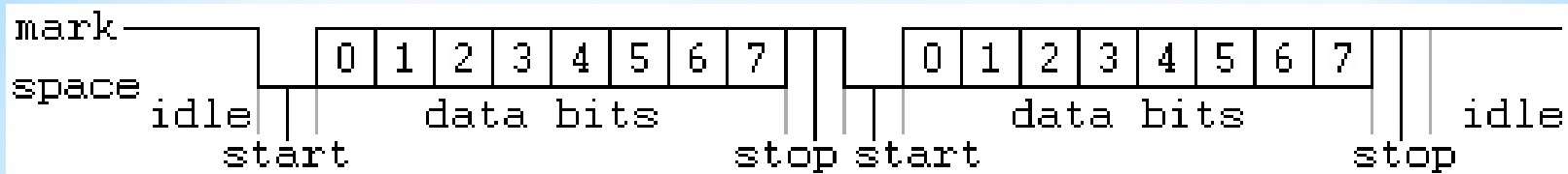
FIGURE 16-2: ASYNCHRONOUS TRANSMISSION
