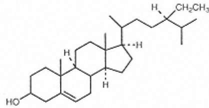
Sitosterol (24- \alpha -ethyl cholesterol) Common plant steroid
