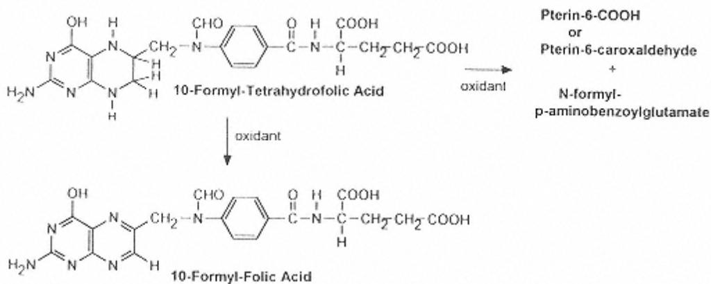
FIGURE 39 Oxidative degradation of 10-formyl- \text{H}_4 folate.
