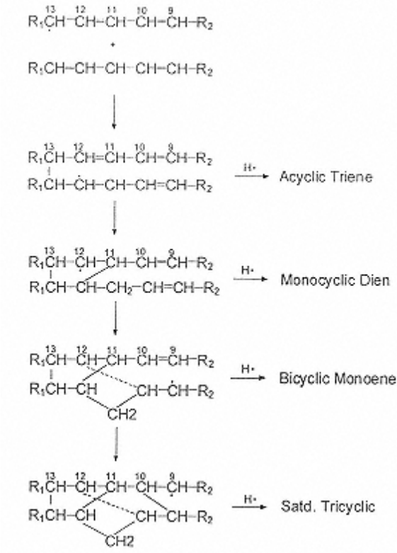
FIGURE 26 Dimerization of linoleate.
