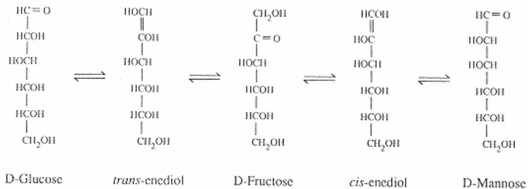
FIGURE 5 Interrelationship of D-glucose, D-mannose, and D-fructose via isomerization.
