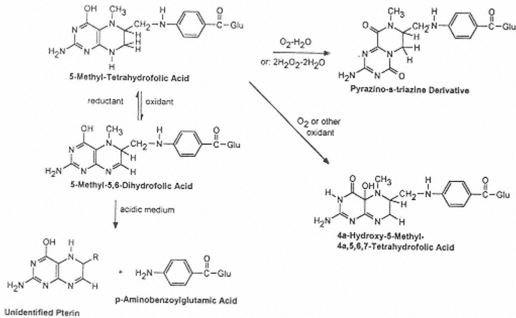
FIGURE 38 Oxidative degradation of 5-methyl- \text{H}_4 folate
