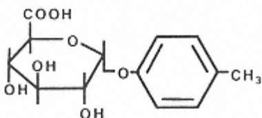
(XXVII) p -Cresyl glucuronide
