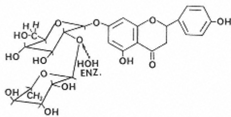
FIGURE 3 Structure of naringin showing site of enzymatic hydrolysis leading to nonbitter derivatives.
