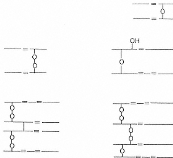
FIGURE 27 Polymerization of acylglycerols.
