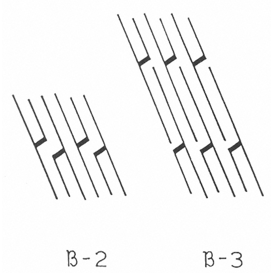
FIGURE 9 Double and triple chair arrangements of form.
