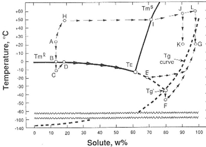
FIGURE 35 State diagram of a binary system showing possible paths for freezing ABCDEF (unstable sequence ABCDE ; stable sequence ABCDEF ), drying (unstable sequence AHIJK ; stable sequence AHIJLG ) and freeze drying ABCDEF (unstable sequence ABCDEG ; stable sequence ABCDEF ). Temperatures during drying are lower than would occur in practice to facilitate entry of data on the graph. Assumptions stated in Figure 25 apply here.
