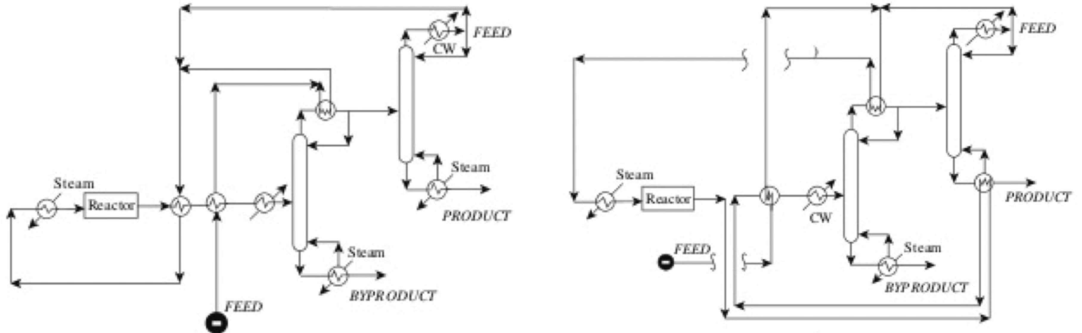
Figure 1.6 A different reactor design not only leads to a different separation system but additional possibilities for heat integration. (From Smith R and Linnhoff B, 1988, Trans IChemE ChERD , 66: 195 by permission of the Institution of Chemical Engineers).
