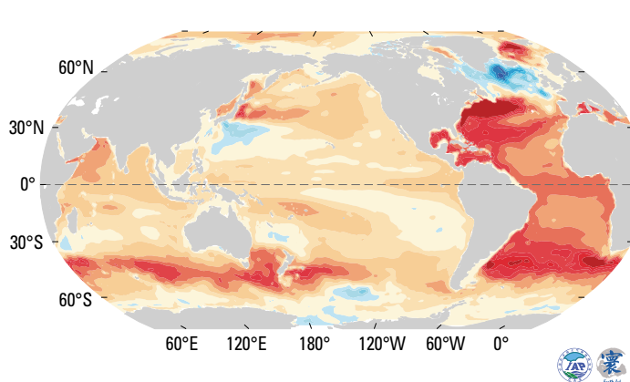
Figure 5. Observed upper 2000 m OHC trend from 1958 to 2023. Source: Data updated from Cheng et al. 25
